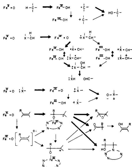
Figure 5. Minimal schemes for the rationalization of oxidative reactions of cytochrome P-450 in terms of perferryl oxygen and electron and hydrogen abstraction. The simplest pathways are shown with heavy arrows.
